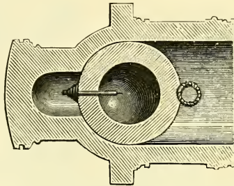
Mortar and Shell requiring Single Ignition only.
